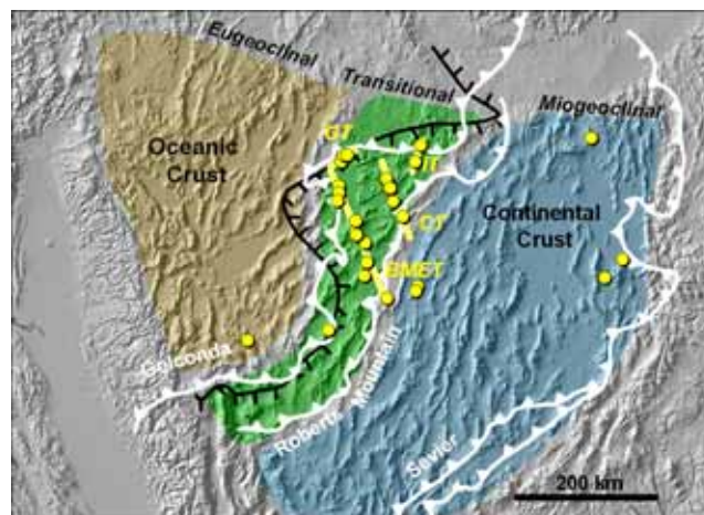
Figure 8. Map of Central Nevada showing the location of Carlin-type deposits and trends, relative to the leading edge of major Paleozoic thrusts (white) and boundary between continental and oceanic crust in the basement (yellow, defined by 87\text{Sr}/86\text{Sr}(i)=0.706 ; from Tosdal et al., 2000). CT = Carlin Trend, BMET = Battle Mountain Eureka Trend, GT = Getchell Trend, IT = Independence Trend. Colored background represents the dominant Paleozoic depositional environment, with favorable, slope-facies (transitional) environment represented in green.
