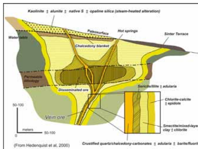
Figure 7. Schematic section showing typical alteration and mineralization patterns in a low sulfidation system. Modified from Hedenquist et al. (2000).
