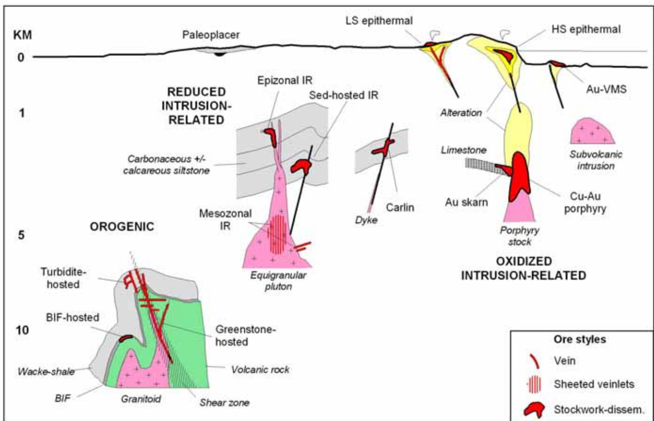
Figure 1: Schematic cross section showing the key geologic elements of the main gold systems and their crustal depths of emplacement. Note the logarithmic depth scale. Modified from Poulsen et al. (2000), and Robert (2004a).
