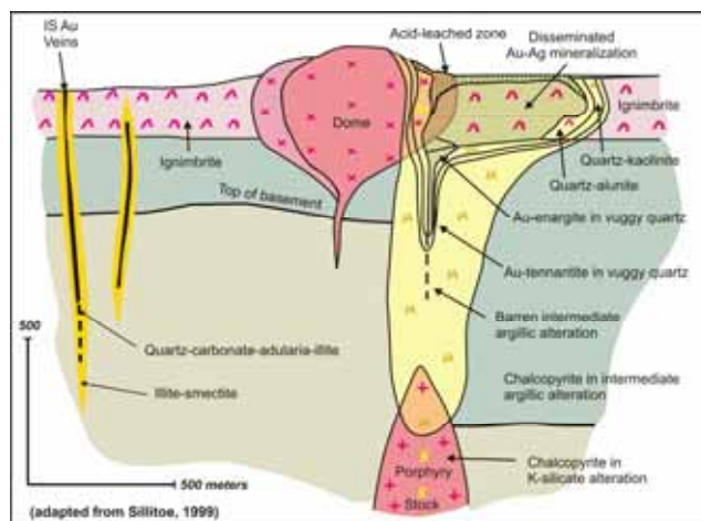
Figure 6. Schematic model of a dome-related HS system above an underlying parent porphyry system. Alteration and Cu sulfide mineral assemblages vary with depth below the paleosurface, which is marked by acid-leached rock of steam-heated origin. Adapted from Sillitoe (1999).
