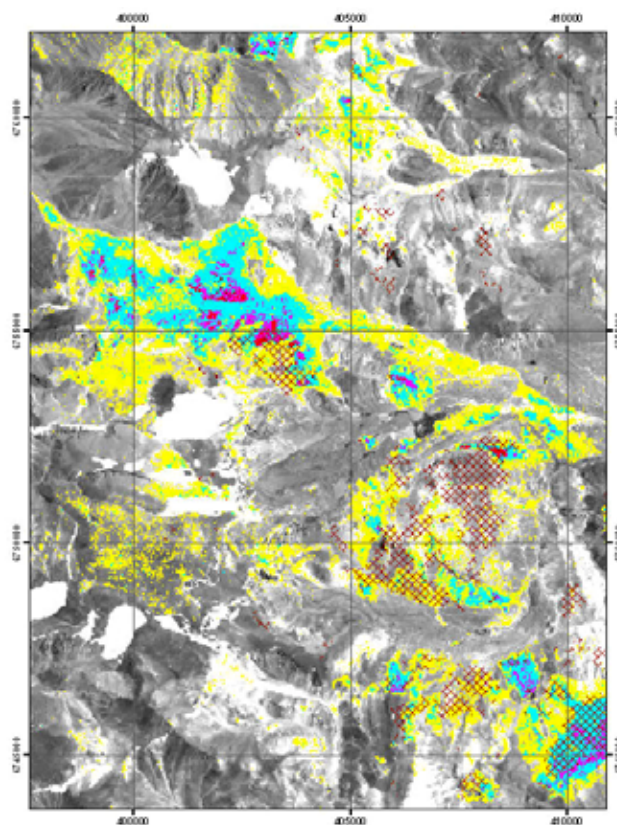
Figure 14. Aster alteration map of the Pascua Lama-Veladero district, Chile. Intense alunite alteration at the core of the system is shown in red to magenta, grading out to argillic alteration in cyan and yellow. Silicification is shown in dark red hatch.
