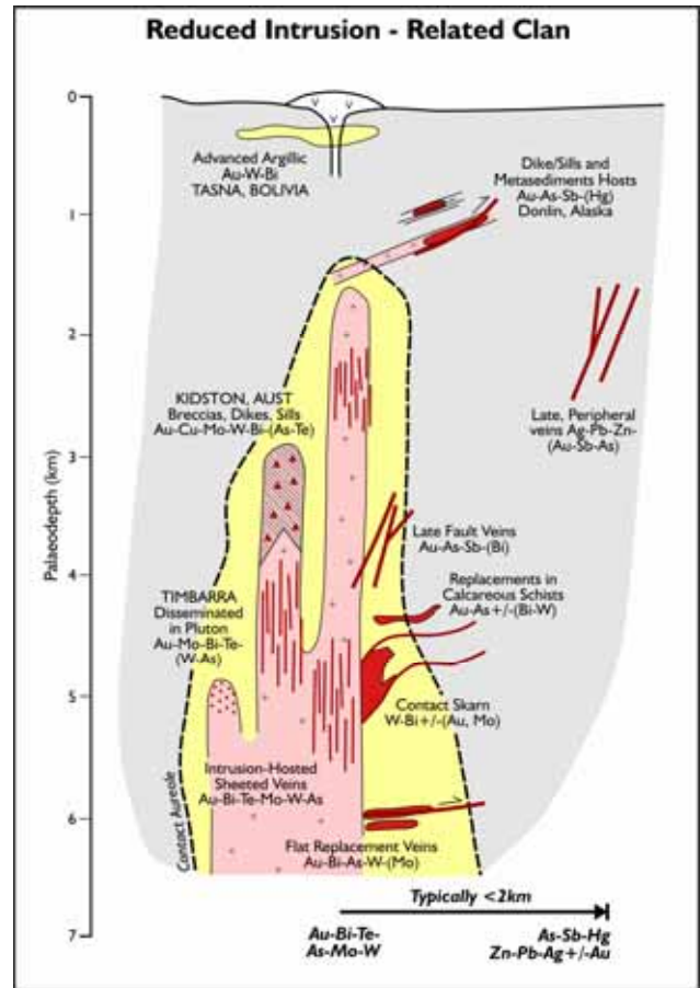
Figure 4. Diagram showing exploration zoning model for intrusion-related gold systems, with an emphasis on systems in Yukon-Alaska but including variations from other intrusion-related gold systems provinces. Modified from Lang et al. (2000).
