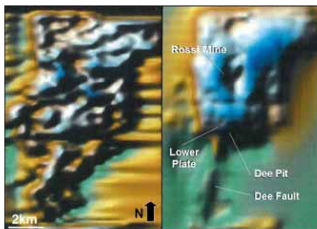
Figure 11. Subsurface conductivity distribution at a depth of 450m obtained from stitching together 2D-TM (left) inversions and 3D inversions (right) of magnetotelluric data over the Dee-Rossi region, Nevada (after Petrick, 2007). Tick spacing is 1km.
